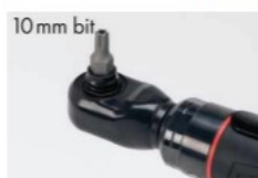
Adapter with 3/8" square drive and 10 mm bit holder
