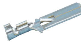
Spade Male Art. No. 00558 991 8 1.5-2.5mm 2
