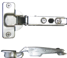
100° Full Overlay - Dowelled
