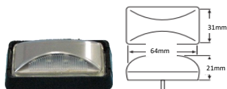
4 LED Number Plate Light
