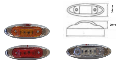
LED Marker Light with Chrome Bezel
