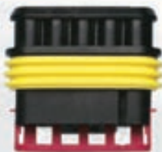
WATERPROOF SOCKET HOUSING TE SUPERSEAL 1.5 SERIES
